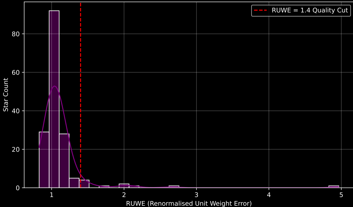
GAPOGEE DR17 Field [203-04] RUWE Distribution (n= 164)
