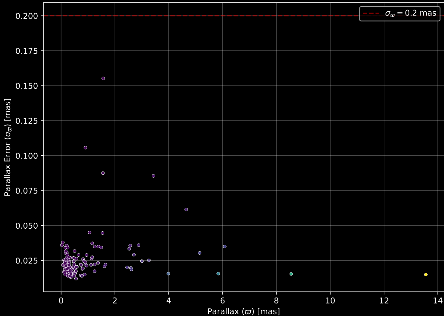
APOGEE DR17 Field: [203-04] Parallax Quality (n= 165)
