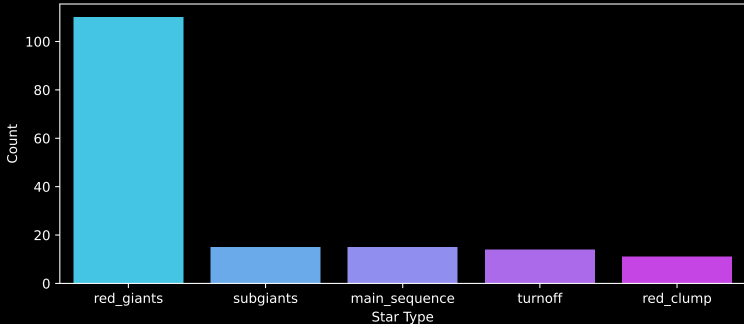
APOGEE DR17 Field: [203-04] Count plot of Star Type
