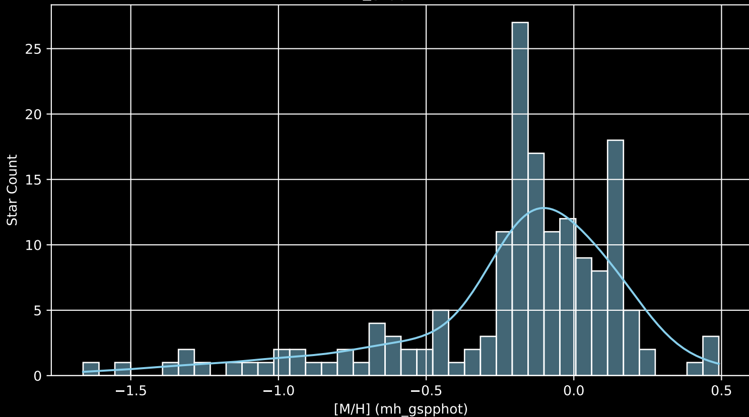
APOGEE DR17 Field: [203-04 [M/H] (mh_gspphot) (n= 164)
