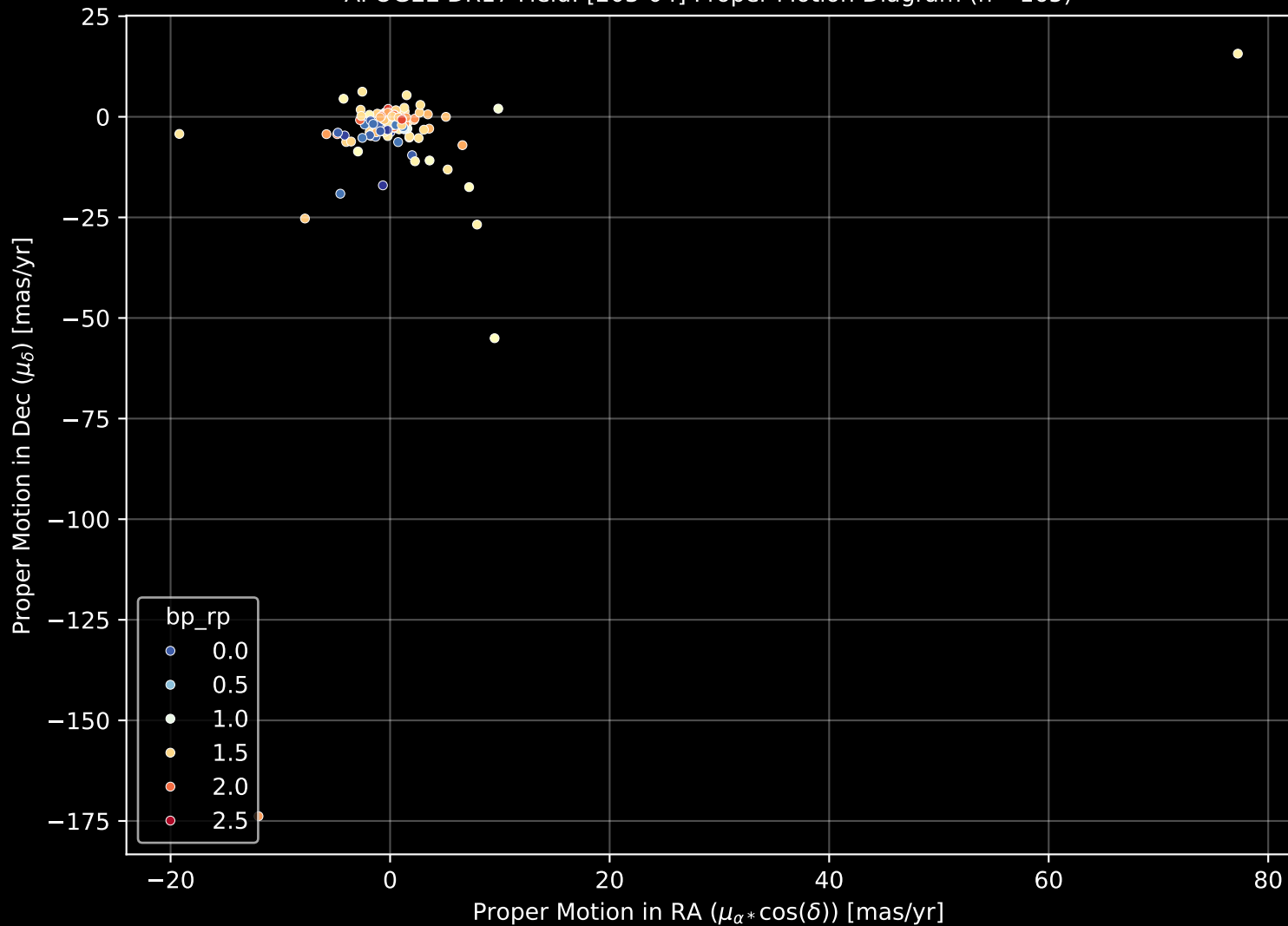
APOGEE DR17 Field: [203-04] Proper Motion Diagram (n= 165)
